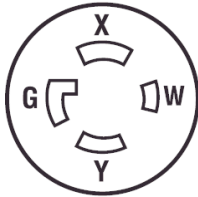
NEMA L14-30R
