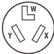
10-30R
